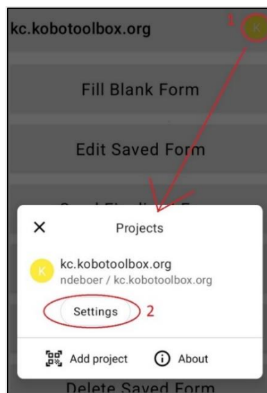
Figure 29. KoBoCollect settings
