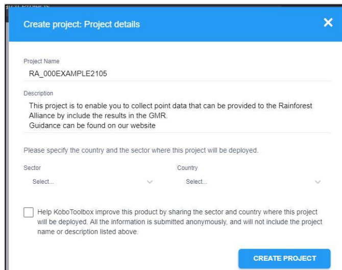
Figure 7. New project
